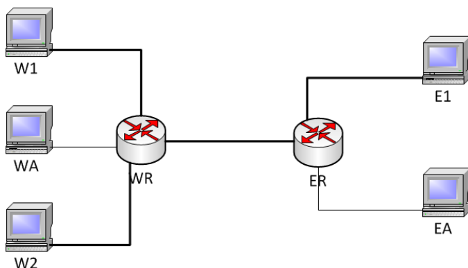
Figure 1. Experiment setup
