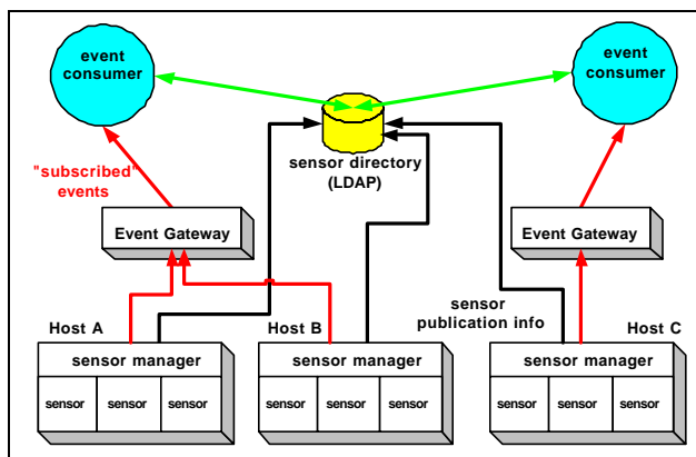
Figure 1: JAMM Components
